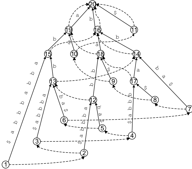
Figure 1. A graph induced from the suffix tree of string ababbabbba\$ . Solid edges represent edges of the suffix tree. The dashed edges represent suffix links.
