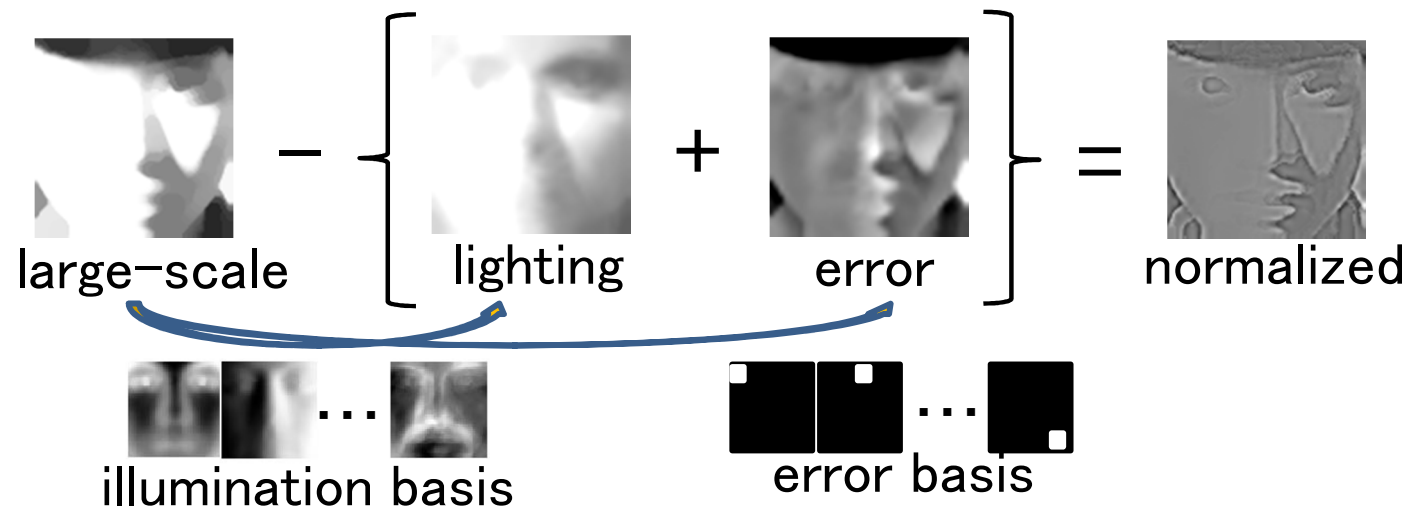
Error term for large-scale feature normalization
